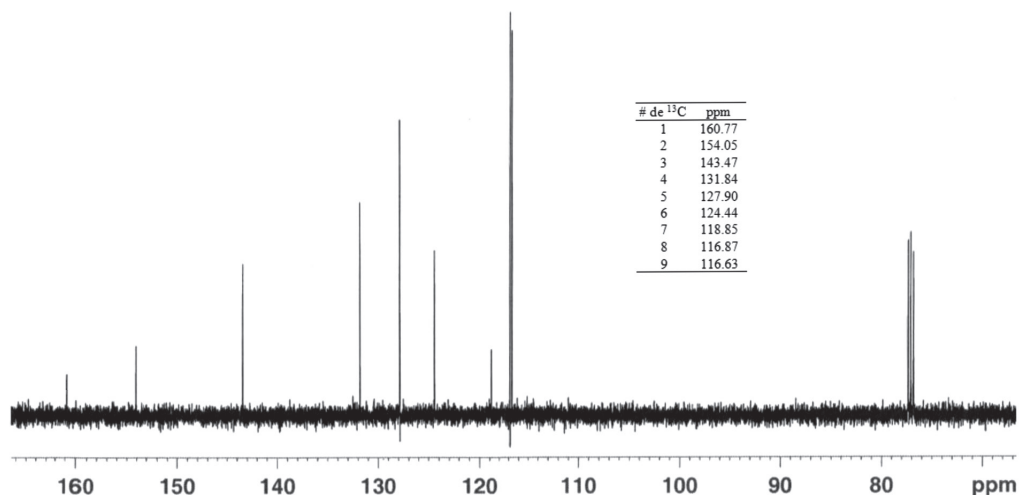
Fig. 3. ^{13}\text{C} -NMR spectrum of compound A of the ascidian R. birkelandi dissolved in \text{CDCl}_3 , performed on a NMR Bruker Avance 500 MHz
