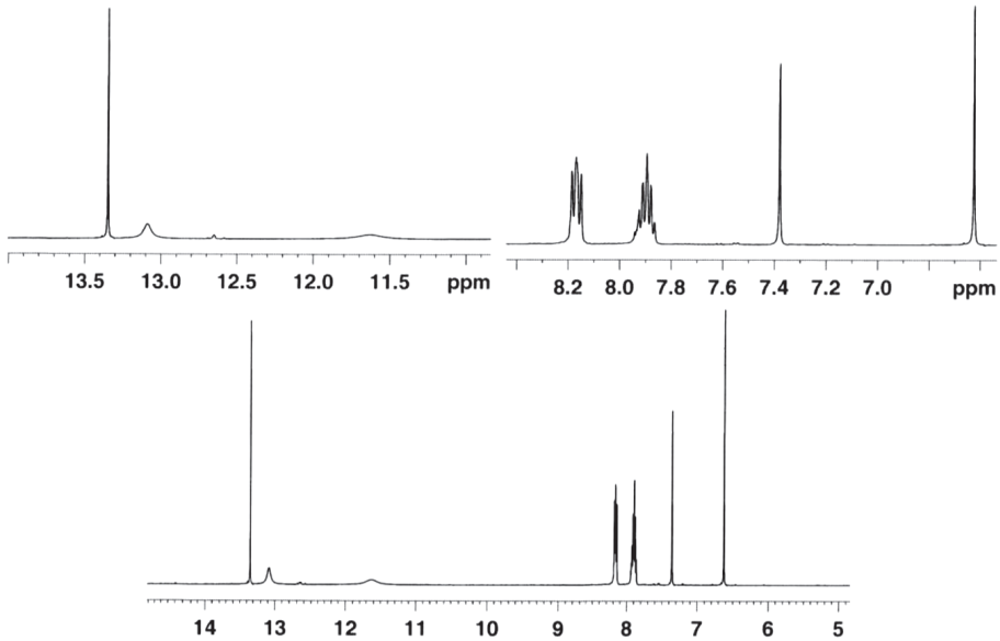
Fig. 8. 1 H-NMR spectrum of compound B of the ascidian R. birkelandi dissolved in DMSO-d 6 , conducted in an NMR Bruker Avance 500 MHz
